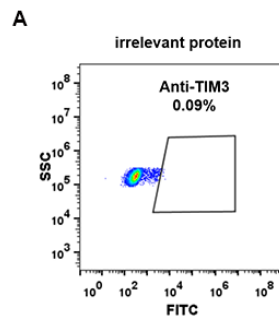
Figure 2. Expi 293 cell line transfected with irrelevant protein (A) and human TIM3 (B) were surface stained with Rabbit anti-TIM3 monoclonal antibody 1µg/ml (clone: DM82) followed by Alexa 488-conjugated anti-rabbit IgG secondary antibody.
