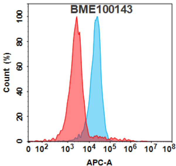
Figure 1. MASP2 protein is highly expressed on the surface of Jurkat cell membrane. Flow cytometry analysis with 15\ \mu\text{g}/\text{mL} Anti-MASP2(narsoplimab biosimilar) mAb (28135) (Blue histogram) or isotype control mAb (Red histogram) on Jurkat cells.
