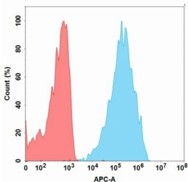
Figure 1. Flow cytometry analysis with 1 \mu\text{g}/\text{mL} Anti-NKG2A (monalizumab biosimilar) mAb (28088) on Expi293 cells transfected with Human NKG2A protein and Human CD94 protein (Blue histogram) or Expi293 transfected with irrelevant protein (Red histogram).
