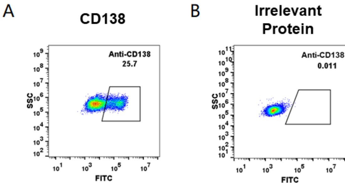
Figure 1. HEK293 cell line transfected with irrelevant protein (B) and human CD138 (A) were surface stained with anti-CD138 neutralizing antibody 1\mu\text{g}/\text{ml} (indatuximab) followed by Alexa 488-conjugated anti-human IgG secondary antibody.
