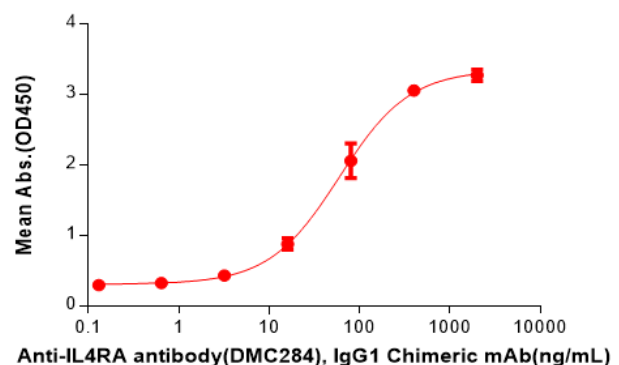
Figure 2. ELISA plate pre-coated by 2 µg/ml (100 µl/well) Human IL4RA Protein, hFc Tag(11593) can bind Anti-IL4RA antibody(DMC284), IgG1 Chimeric mAb in a linear range of 16.0-400 ng/mL.
