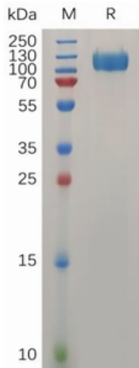
Figure 1. Human IFNAR1 Protein, mFc Tag on SDS-PAGE under reducing condition.
