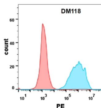
Figure 2. Flow cytometry analysis with CD7 (DM118) on Expi293 cells transfected with human CD7 (Blue histogram) or Expi293 transfected with irrelevant protein (Red histogram).
