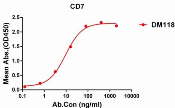
Figure 1. ELISA plate pre-coated by 1\ \mu\text{g/ml} ( 100\ \mu\text{l/well} ) Human CD7 protein, mFc-His tagged protein 11276 can bind Rabbit anti-CD7 monoclonal antibody (clone: DM118) in a linear range of 0.2-60 ng/ml.
