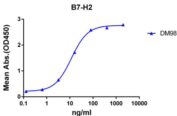
Figure 1. ELISA plate pre-coated by 2 µg/ml (100 µl/well) Human B7-H2 protein, mFc-His tagged protein 11157 can bind Rabbit anti-B7-H2 monoclonal antibody ( clone: DM98) in a linear range of 3.2-80 ng/ml.
