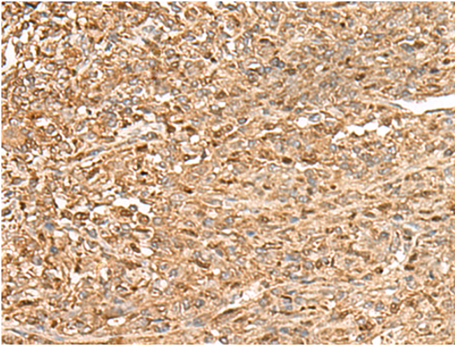
Immunohistochemistry analysis of paraffin embedded Human liver cancer tissue using 212519(ZC3H7A Antibody) at a dilution of 1/50(Cytoplasm).
