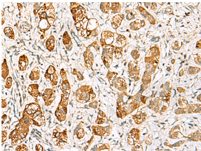
Immunohistochemistry analysis of paraffin embedded Human liver cancer tissue using 218862(RIMS3 Antibody) at a dilution of 1/60(Cytoplasm).
