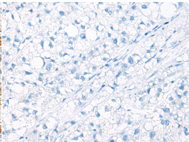
In comparison with the IHC on the left, the same paraffin-embedded Human liver cancer tissue is first treated with the fusion protein and then with 218862(Anti-RIMS3 Antibody) at dilution 1/60.
