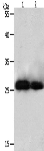
Gel: 10%SDS-PAGE, Lysate: 40 µg; Lane 1-2: HeLa cells, 293T cells; Primary antibody: 213722(PRDX3 Antibody) at dilution 1/800; Secondary antibody: Goat anti rabbit IgG at 1/8000 dilution; Exposure time: 20 seconds
