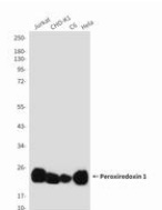
Western blot analysis of Peroxiredoxin 1 (6A6) in urkat, CHO-K1, C6, HeLa lysates using Peroxiredoxin 1 (6A6) antibody
