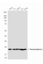
Western blot analysis of Prdx 1 in T47D, 3T3, COS7, C6 and HeLa lysates using Prdx 1 antibody.
