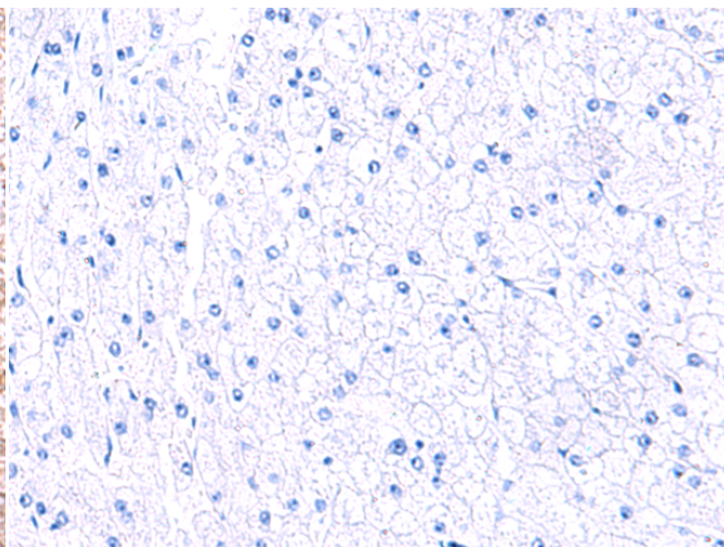
In comparison with the IHC on the left, the same paraffin-embedded Human liver cancer tissue is first treated with the fusion protein and then with 218802(Anti-PDRG1 Antibody) at dilution 1/75.
