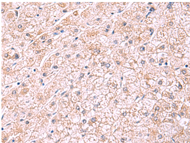
Immunohistochemistry analysis of paraffin embedded Human liver cancer tissue using 218802(PDRG1 Antibody) at a dilution of 1/75(Cytoplasm).
