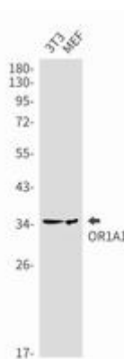
Western blot analysis of OR1A1 in 3T3, MEF lysates using OR1A1 antibody.
