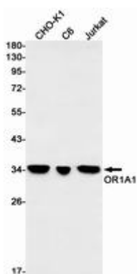
Western blot analysis of OR1A1 in CHO-K1, C6, Jurkat lysates using OR1A1 antibody.
