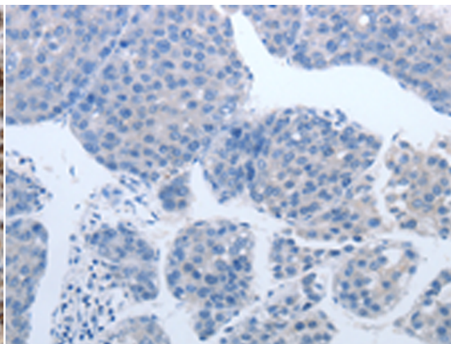
In comparison with the IHC on the left, the same paraffin-embedded Human liver cancer tissue is first treated with the fusion protein and then with 216643(Anti-MCM3 Antibody) at dilution 1/30.
