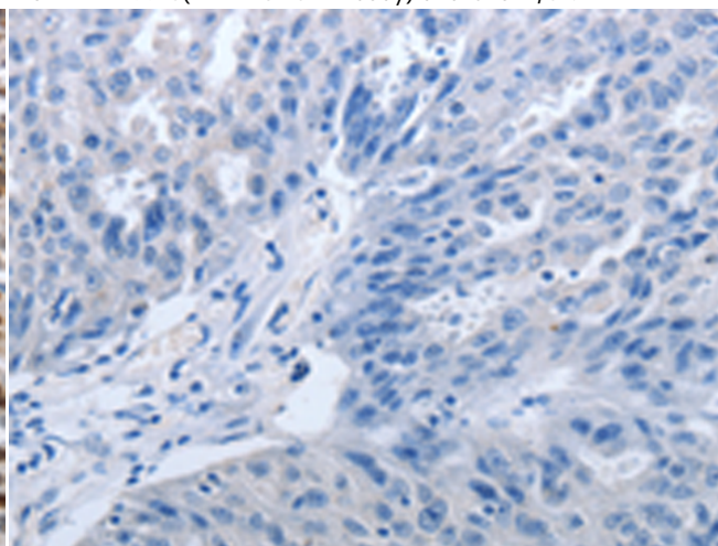
In comparison with the IHC on the left, the same paraffin-embedded Human ovarian cancer tissue is first treated with fusion protein and then with D220966(Anti-MCM3 Antibody) at dilution 1/30.
