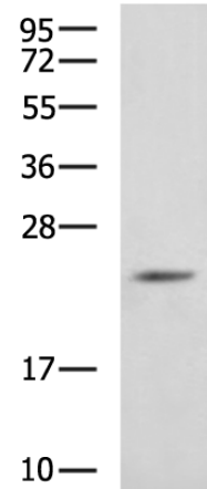
The image on the left is immunohistochemistry of paraffin-embedded Human colorectal cancer tissue using 217440(Anti-FGF18 Antibody) at a dilution of 1/70.
