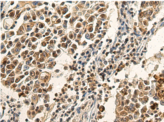
Immunohistochemistry analysis of paraffin embedded Human lung cancer tissue using 219333(CD2BP2 Antibody) at a dilution of 1/120(Nucleus).
