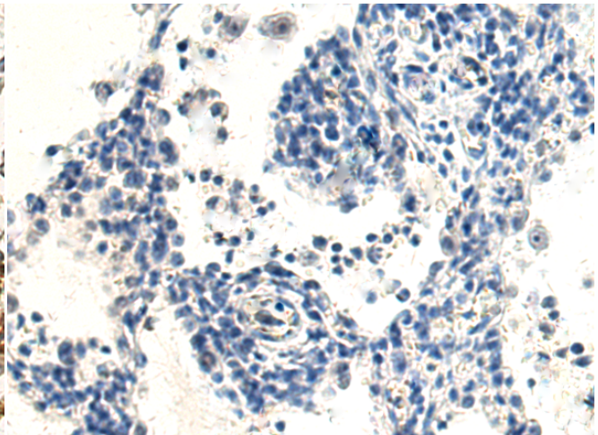
In comparison with the IHC on the left, the same paraffin-embedded Human lung cancer tissue is first treated with the fusion protein and then with 219333(Anti-CD2BP2 Antibody) at dilution 1/120.
