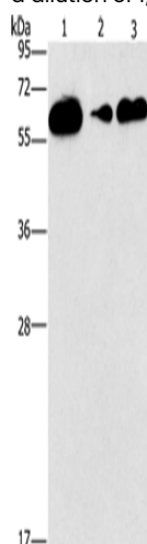
Gel: 10%SDS-PAGE, Lysate: 40 µg; Lane 1-3: Raji cells, PC3 cells, Iovo cells; Primary antibody: 217262(CD27 Antibody) at dilution 1/727; Secondary antibody: Goat anti rabbit IgG at 1/8000 dilution; Exposure time: 1 minute
