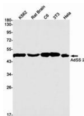
Western blot analysis of AdSS 2 in K562, rat Brain, C6, 3T3, HeLa lysates using AdSS 2 antibody.
