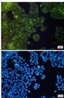
Immunocytochemistry analysis of AdSS 2 (green) in HeLa using AdSS 2 antibody, and DAPI (blue)
